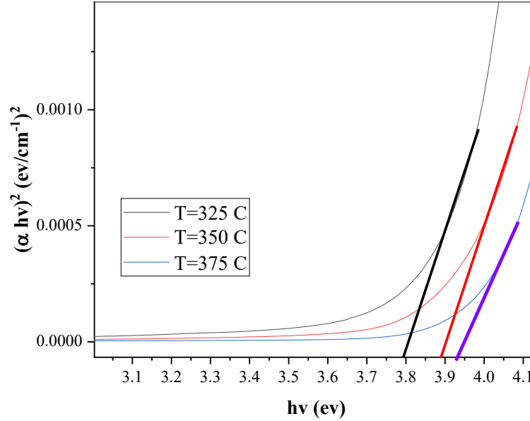
Figure 6: Tauc plots (\alpha hv)^2 vs. h\nu for \text{SnO}_2 thin films prepared at 325 °C, 350 °C, and 375 °C. The plots reveal a direct band gap nature, with the energy gap increasing from 3.80 eV to 3.94 eV as deposition temperature rises.
