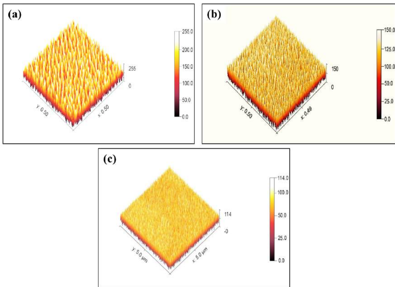
Figure 3: Atomic force microscopy (AFM) images of SnO 2 thin films synthesized at (a) 325 °C, (b) 350 °C, and (c) 375 °C, showing temperature-dependent changes in surface topography.
