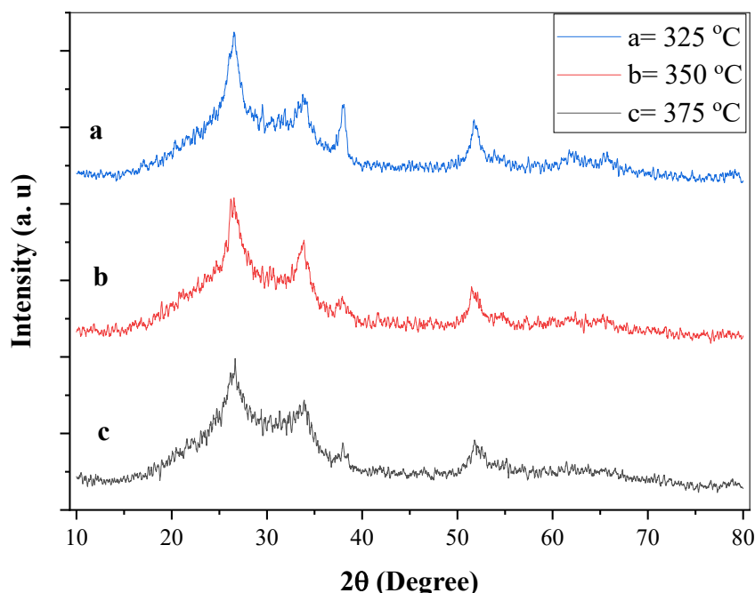
Figure 1: X-ray diffraction (XRD) patterns of SnO 2 thin films synthesized at 325 °C (blue), 350 °C (red), and 375 °C (black). All samples exhibit the rutile tetragonal phase of SnO 2 . Peak intensity and sharpness decrease with increasing deposition temperature, indicating reduced crystallinity and increased structural disorder
