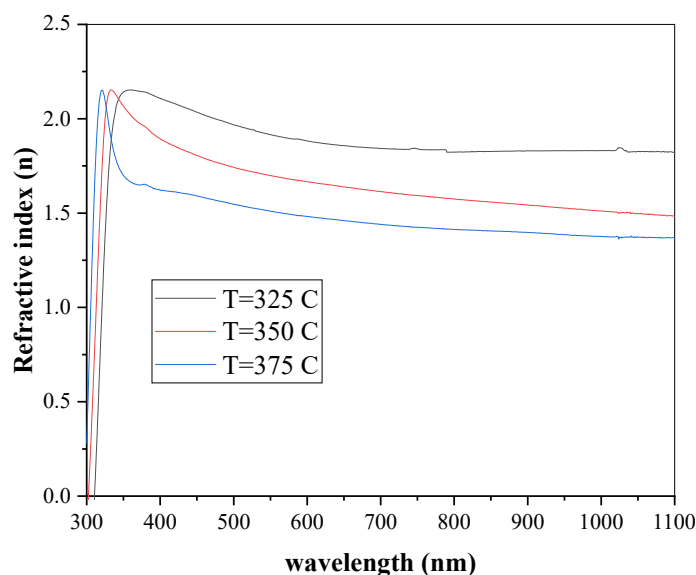
Figure 7: Refractive index ( n ) values of SnO 2 thin films prepared at 325 °C, 350 °C, and 375 °C by the chemical pyrolysis method at a precursor concentration of 0.02 M.
